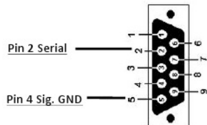
Female DB9 for PC Port
